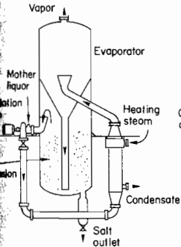
Evaporator crystallizer
