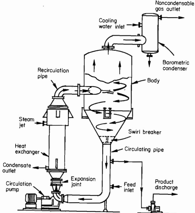
Fig. 8 Forced-circulation (evaporative) crystallizer.
